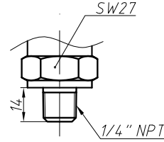
1/4" NPT
